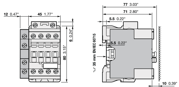
AF09, AF12, AF16 + CAL4-11 2-poliger Hilfskontaktblock
